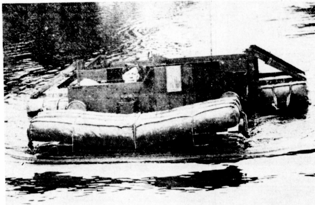
WHEN A GUN SWIMS—Kapak floats lend buoyancy to this heavy Bren gun carrier, "swimming" across a river in the North of England. Rotating tracks are used for steering across the water. Demonstration at military school.
