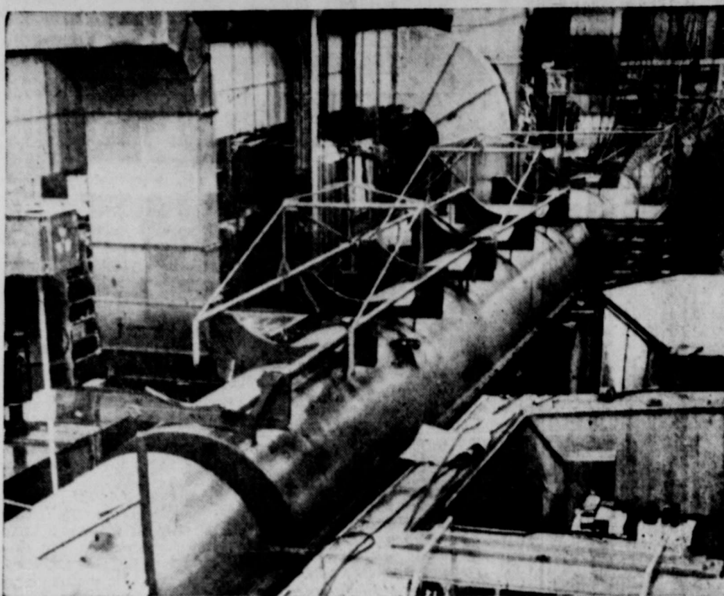
IT'S THE "LINAC," the world's most powerful straight line atom smasher, nearing completion at the University of Minnesota. The long tube is the business part. The "linac" is being built under an Atomic Energy commission grant of $1,800,000. (International Soundphoto)
