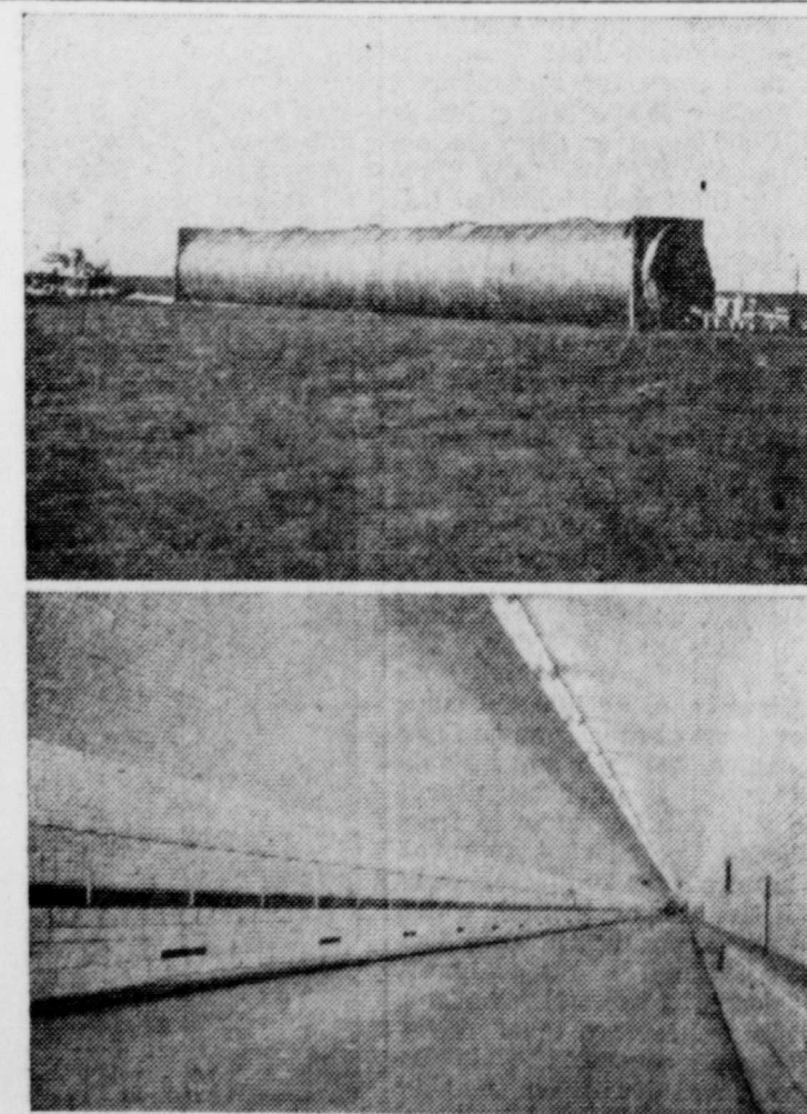
TUNNEL TUBE —New achievements in tunnel construction were marked by the completion of the Baytown-LaPorte tunnel, longest in Texas. The 3009-foot underwater structure is an impressive example of engineering with its well-lighted interior, bottom. A giant steel tube, top, one of nine similar sections forming a protective liner, is shown being floated down Galveston Bay to be sunk, top photo. About 8,500,000 pounds of steel were used.
