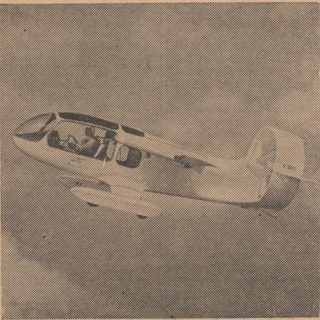
FLYING MARVEL was designed for study of low-speed flying. It is powered by an engine which weighs only 136 pounds but develops 317 horsepower.
