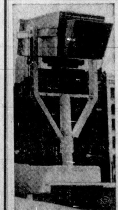
BRIDGE TENDER—There's a television camera, complete with windshield wiper, installed in the all-weather enclosure seen above. The camera is at one end of the Monroe St. bridge in Chicago. There used to be a bridge tender at each end, but with the aid of the TV camera, a single attendant is able to look at the picture screen and see if anyone or a vehicle is on the bridge before raising it to let a ship through.
