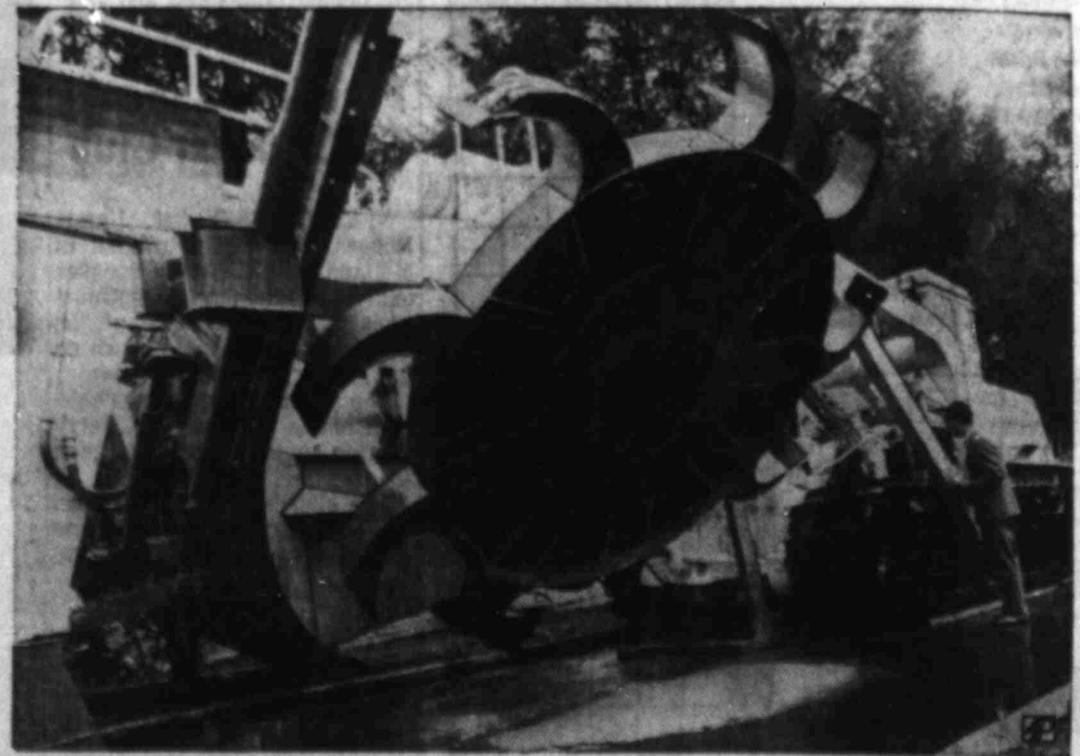
THE BIG DIGGER — The Soviet Union has developed this giant double rotor earth excavator which is being used in the construction of the North Crimea irrigation canal.
