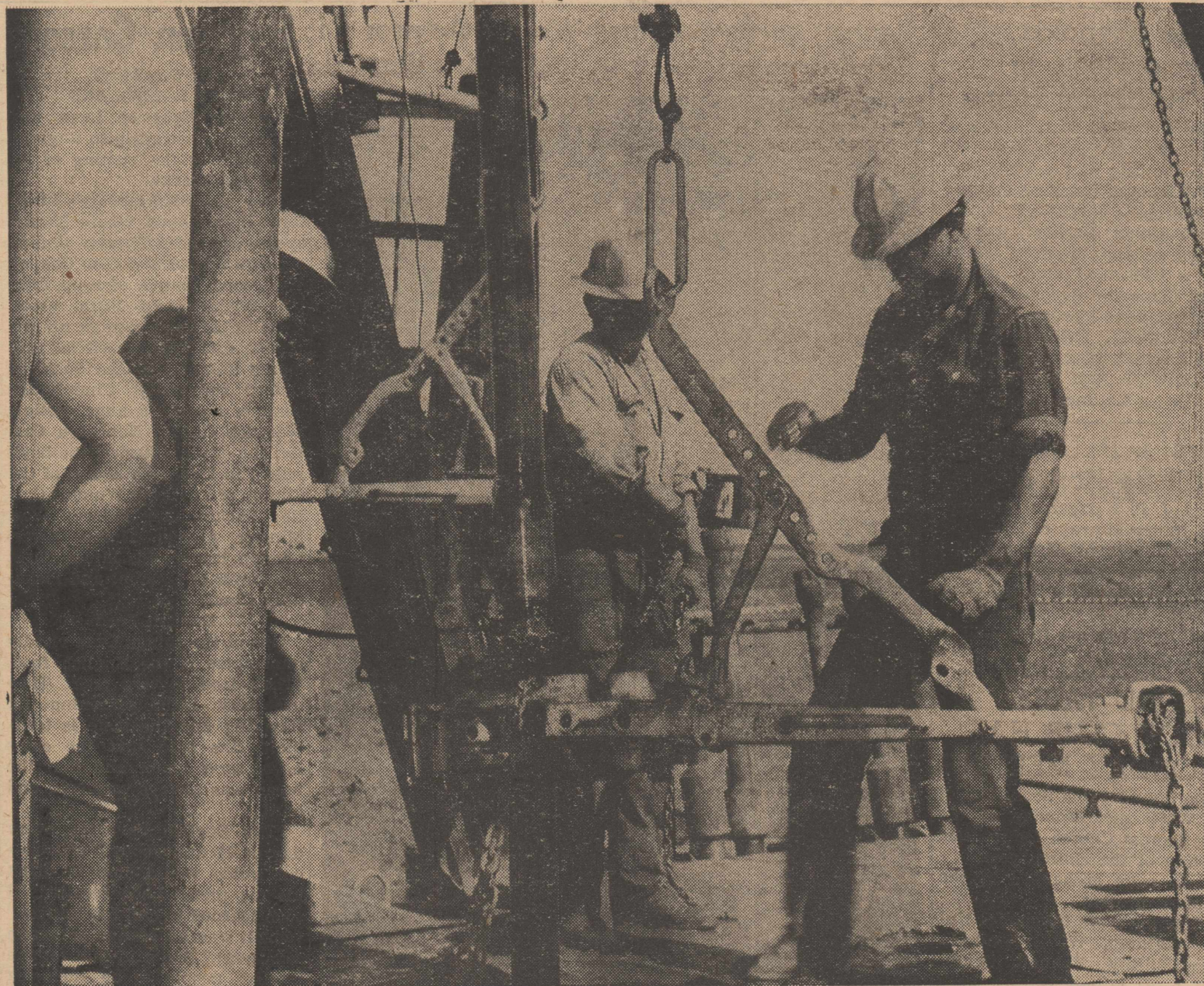
HART CAMP has a new oil well in the process of being drilled just south of the Hart Camp store and gin. It is going down on the M. V. Kesey place. Mr. Kesey lives at Littlefield, A. J. Little, left hand photo, tool pusher for the Montex Drilling Company, said the San Andres formation will be tested. That is the same formation which is yielding oil at Littlefield. The well is being drilled for the W. A. Moncrief Company of Fort Worth. Another wildcat well which was plugged recently about a mile northwest of the present site is reported to have been a dry hole in the Glorietta formation. The men above are shown working on the rig. (S-Ps)
