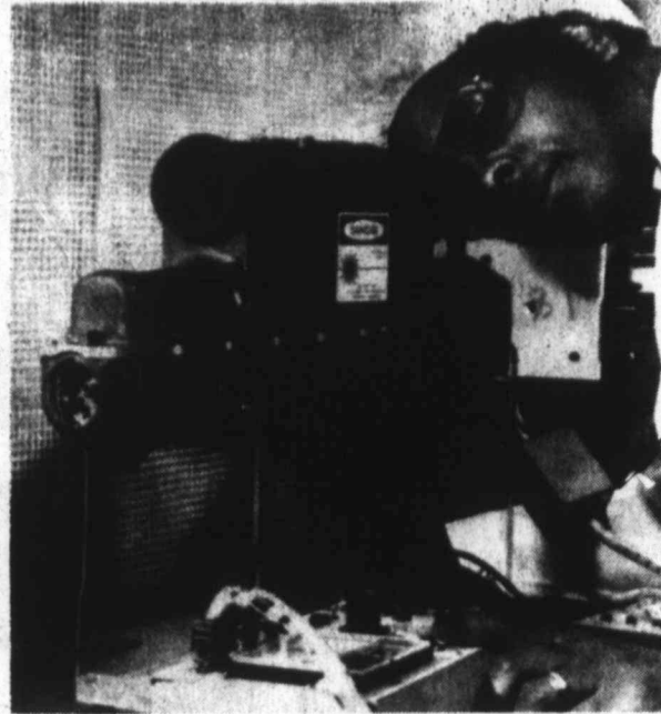
ON TARGET! — Engineer Douglas Chism peers through U.S. Army's new Laser Target Designator recently during testing at Hughes Aircraft Company's electro-optical and data systems group, at Culver City, Calif. The first such device to be produced for the army, the laser target designator can guide homing weapons to targets, mark troop positions, or mark sites for aerial supply drops. Hughes will manufacture 152 such systems for the Army and 25 more for the Air Force under a U.S. Army Missile Research and Development Command contract in excess of $15 million.
