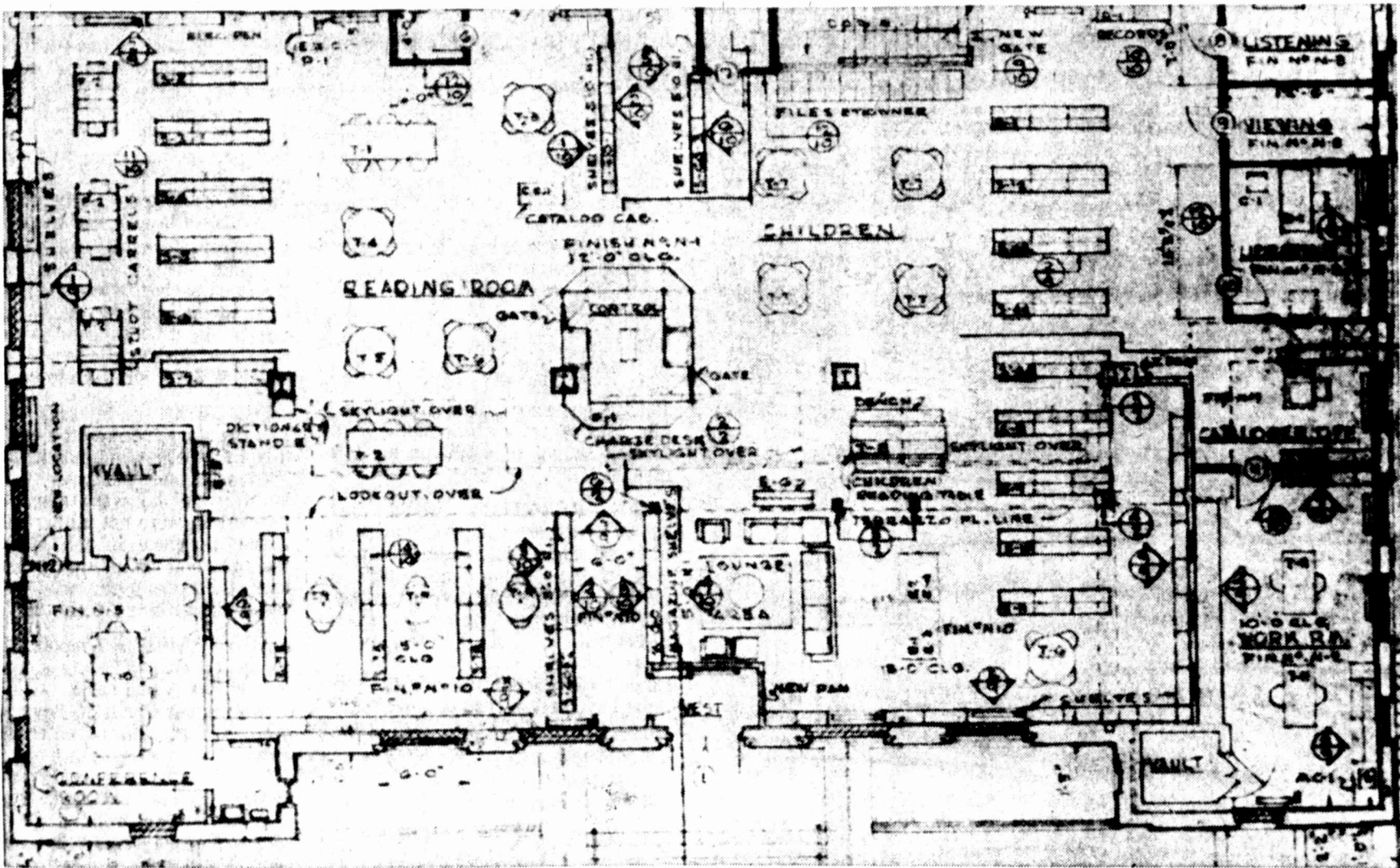
NEW LIBRARY — This is the floor plan of the new Howard County library on which construction should start this week. Kasch Brothers, Inc., was awarded the bid Monday for $63,000 to remodel the old post office into a library. At the bottom of the picture is the Scurry Street entrance.
