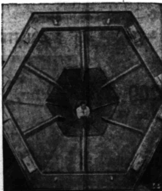
STRONG TOP —Engineer inspects interior of a glass fiber reinforced church spire at Tilbury, Eng. Spire was designed to withstand a wind force of hurricane strength.
