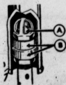
(A) Stainless Steel Balls on brass valve seats make a perfect seal in the check valves and plunger.
