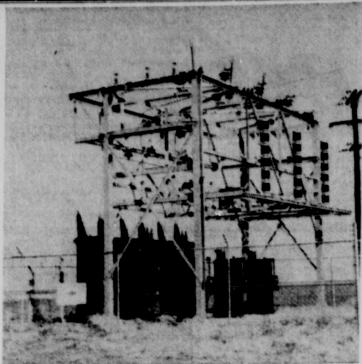
REA SUBSTATION—This Perryton substation of the North Plains Electric Cooperative will be energized on Tuesday, February 26, thus bringing much more electrical power to residents of this area. The substation will give adequate power to subscribers and shorten the distribution lines so that better service can be given. This substation is located five miles south of Perryton.
