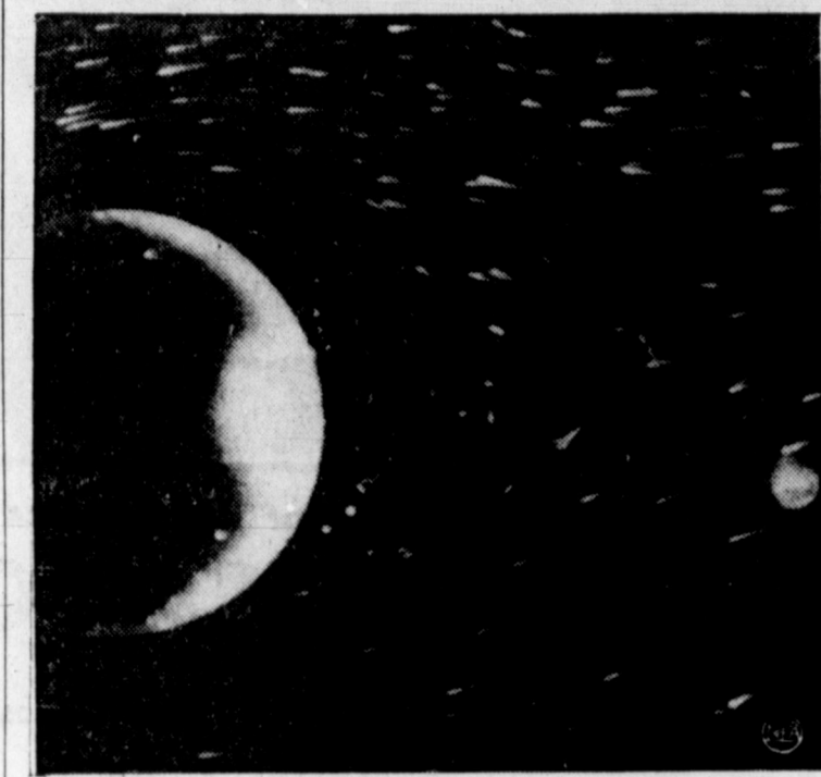
TUNNEL "MOON" —What looks like a time-lapse picture of the moon against a background of blurry stars is actually a steel sphere and the patterns formed as water flows around it inside a new water tunnel at the Westinghouse Research Laboratories in Pittsburgh, Pa. The tunnel, containing 13 tons of water moving at 8,000 gallons a minute, is used to study similar flow patterns past more complicated structures, such as the turbine blade of a jet engine.
