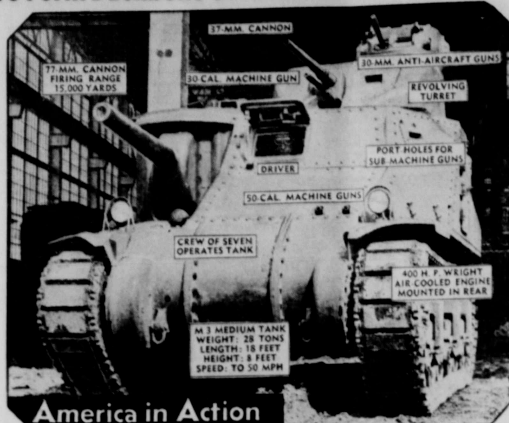
M3, the army's new 28-ton tank, is heavily armed and is designed for speed and maneuverability as well as power.
