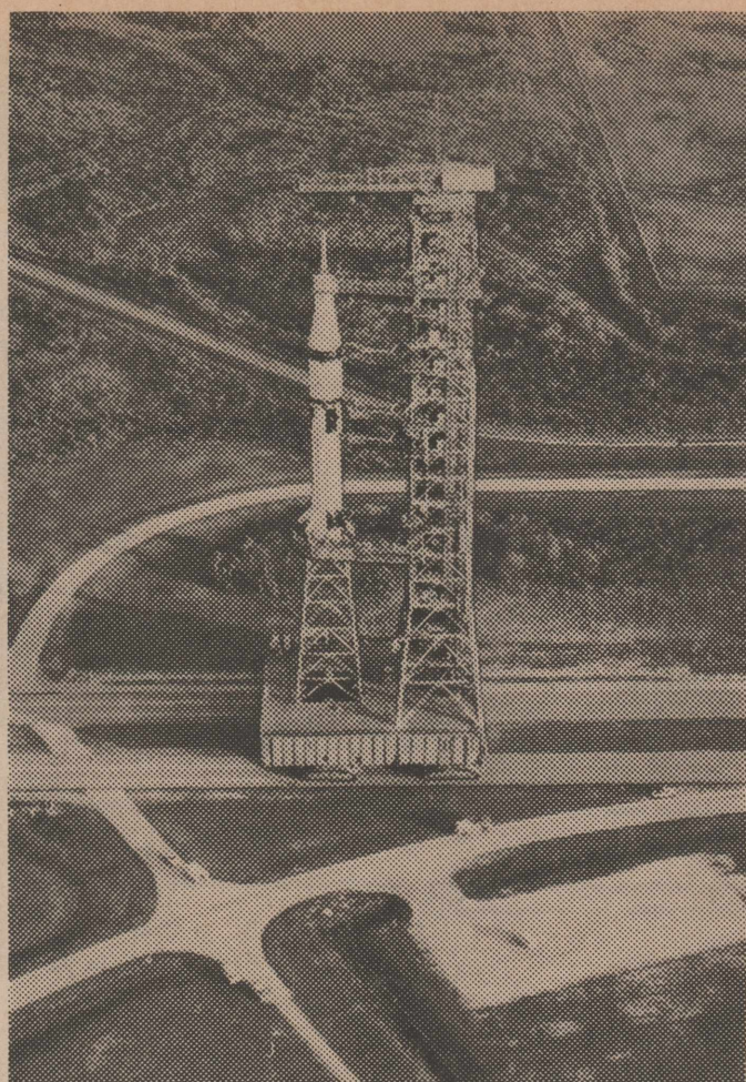
MAKING TRACKS to its launch site at Kennedy Space Center, Fla., is the gigantic Saturn rocket which will send the first crew to the Skylab orbital workshop in May. The crew will blastoff 24 hours after the Skylab is launched into space.
