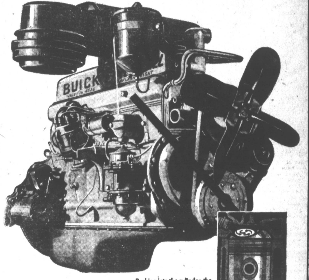
Rushing into the cylinder, the fuel charge strikes the Turbo-Top piston—swirls into a tiny cyclone of terrific turbulence that gives a mighty power-push to the ignited fuel.
