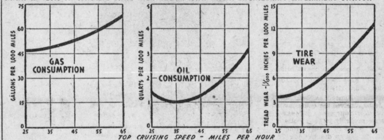
CHART 1. TESTS ON CONCRETE STATE HIGHWAYS IN IOWA - IOWA ENGINEERING EXPERIMENT STATION
