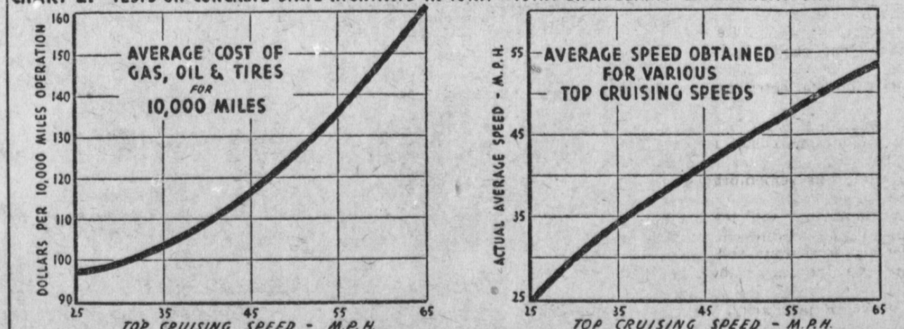
CHART 2. TESTS ON CONCRETE STATE HIGHWAYS IN IOWA - IOWA ENGINEERING EXPERIMENT STATION
