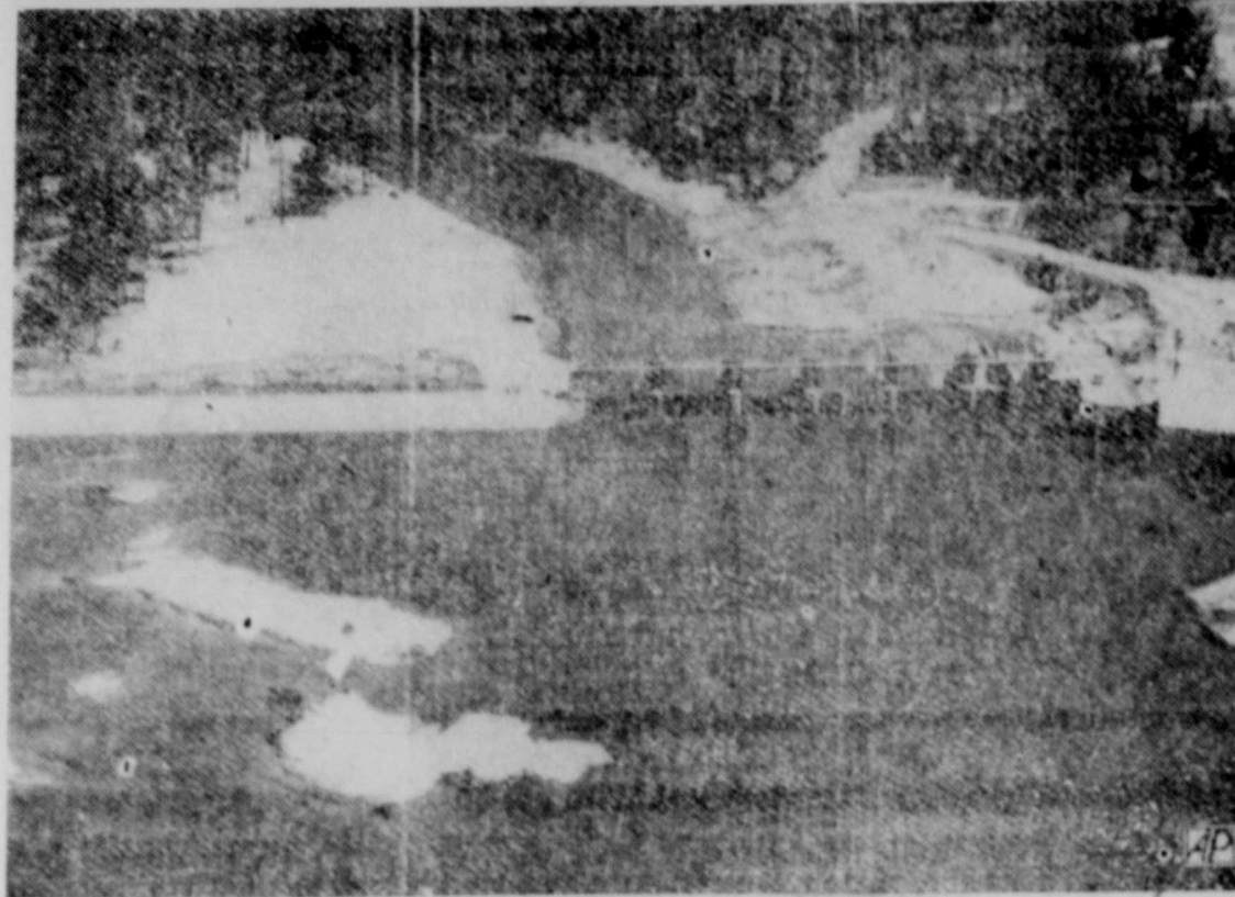
TOWN BLUFF DAM —The Town Bluff dam on the Neches River 50 miles north of Beaumont will be opened officially in a public celebration (May 5). The dam impounds the largest fresh water lake in East Texas. It is 14 miles long and five miles wide. This aerial photo shows the reservoir fillin behind the six-gate spillway. (L.P. Photo)
