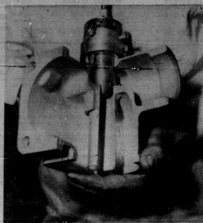
A CUTAWAY VIEW shows the Y-Z Dual Load Fuel Valve in operating position. The valve is designed, patented and manufactured by Y-Z Engineers Service.
