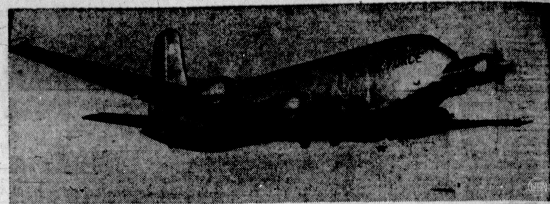
PULLED BY THE NOSE —"Schnozzola" could be the name for this Air Force C-124 Globemaster. It sports a Pratt and Whitney T-37 engine in its nose. The company is using the aircraft as a test bed for the new propeller-turbine engine intended for transcontinental transport of the Air Force. The entire forward structure of the huge plane had to be altered for the testing at East Hartford, Conn.
