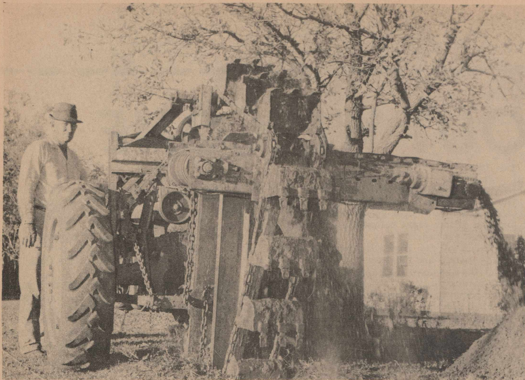
WATER SUPT. W. F. Williamson has been putting in some steady hours the last several days in making this ditch-digger perform correctly. Ditches for a two-inch water line are being dug from Ninth Street to the middle of 12th Street. The new water line will replace the one which now lies underneath the highway. Williamson said the new line also would boost water pressure.
