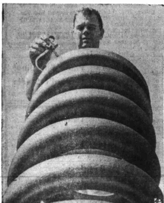
FOR POWER — Technician checks out heavy-duty spring part of giant safety valve, to be installed in an atomic power generating plant being built in Florida.
