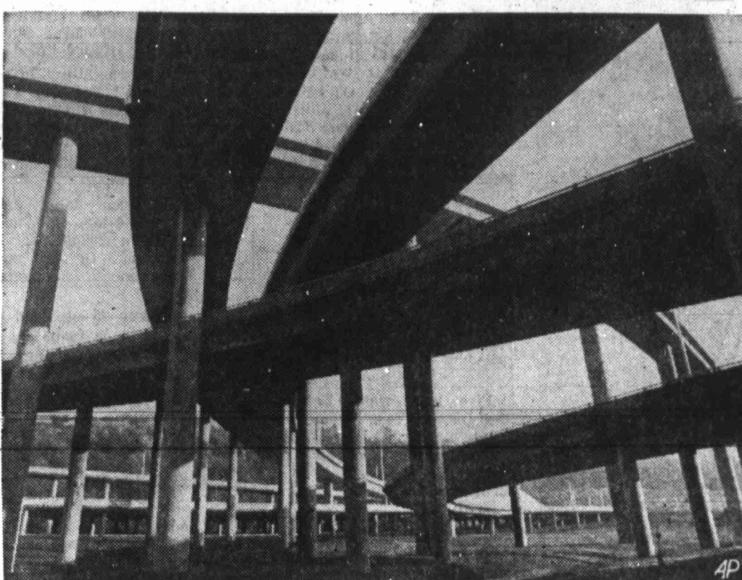
MAZE OF MODERNITY — The concrete twists of the Spokane Street interchange on the Seattle Freeway present a virtual labyrinth to the out-of-town motorist. The interchange is composed of 15 major bridges carrying 17 different traffic movements.
