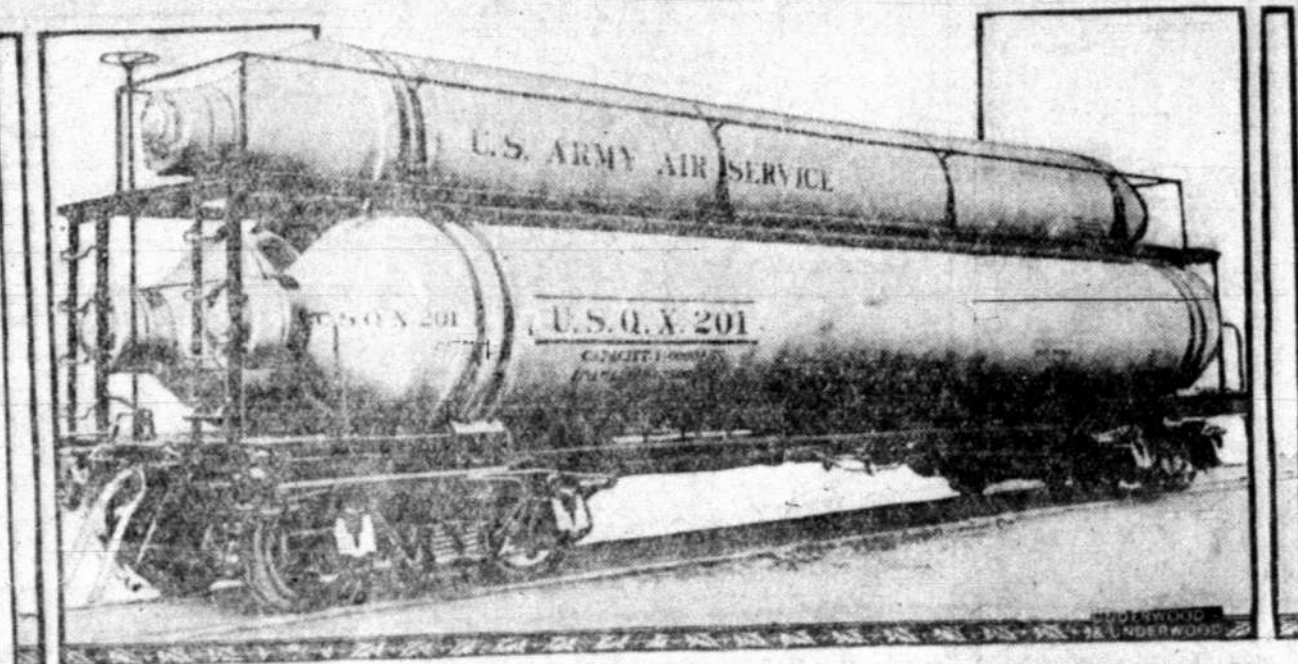
This helium tank car has just been built for the United States air service. Its capacity is 200,000 cubic feet of gas. Under the old system it would take 1,200 small cylinders to fill the 200,000-cubic-foot dirigibles in the air service, and a loss of 15 per cent usually resulted.
