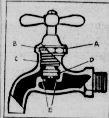
WORKINGS of a compression faucet: (A) cap nut, (B) packing washer, (C) spindle, (D) disk washer, (E) ground seat into which washer fits when faucet is closed.
