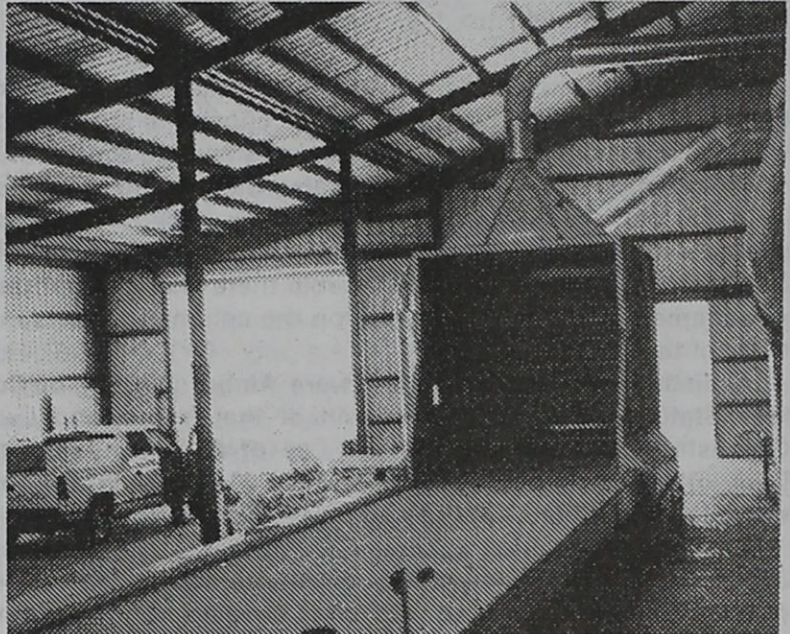
This is the module feeder where the modules are broken up so the cotton can be transported to other parts of the gin. It can handle three modules an hour.
