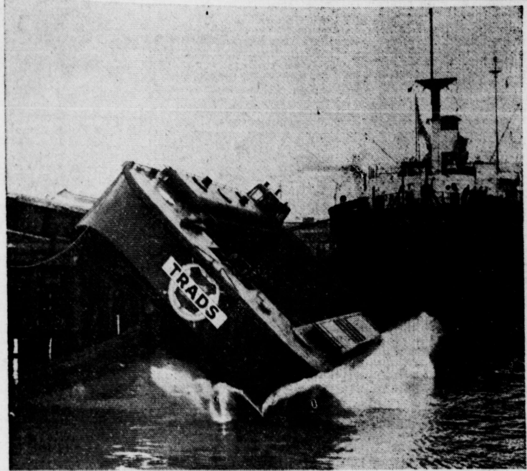
THE BIG SPLASH—The U. S. Army's newest amphibious vehicle is getting into the waters of Puget Sound, at Seattle, Wash., after being pushed off a 12-foot pier. The 60-ton barge, capable of carrying two medium tanks, is undergoing tests for the Army Transportation Corps.
