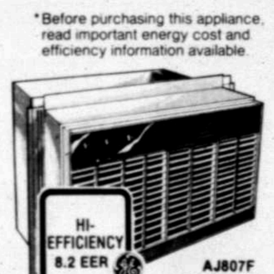
7,300 BTU THINLINE™ ROOM AIR CONDITIONER • 115 Volts, 7.5 Amps • 10 Position Thermostat • 2 Fan/2 Cooling Speeds • Easy-Mount™ Installation
