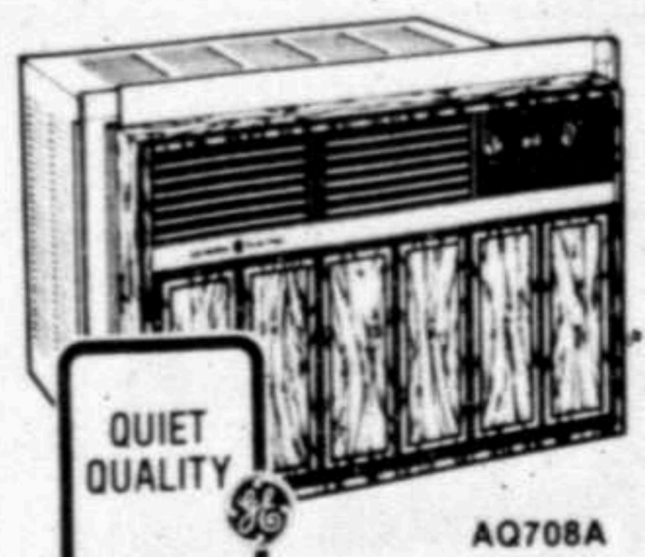
7,600 BTU QUIETAIRE™ HI-EFFICIENCY™ ROOM AIR CONDITIONER • 115 Volts, 9.1 Amps • Ultra Quiet • 10 Position Thermostat • 3 Fan/3 Cooling Speeds • Before purchasing this appliance, read important energy cost and efficiency information available.
