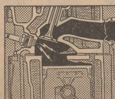
VALVE-IN-HEAD DESIGN
