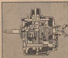
SYNCHRO-MESH TRANSMISSION
