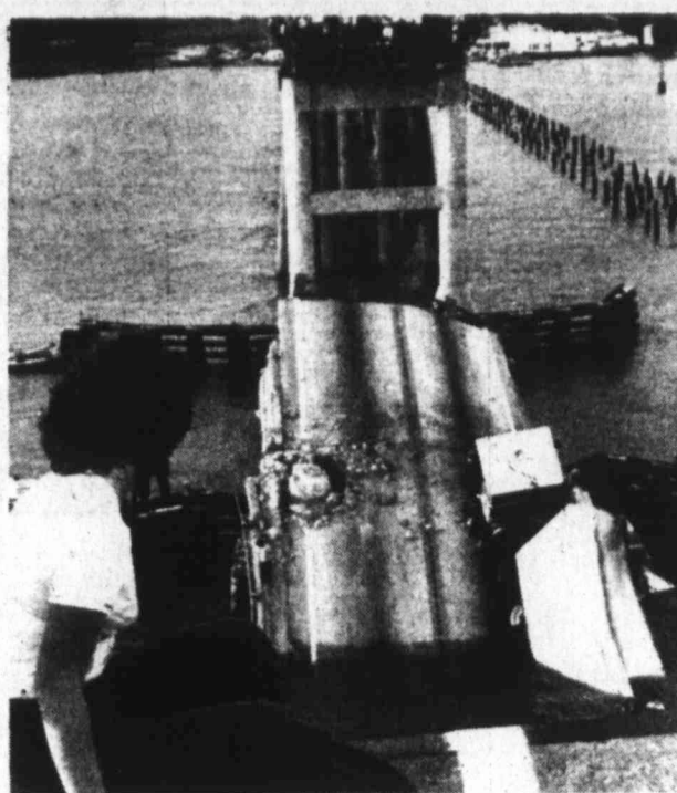
END OF THE LINE — The white line ended here after a barge collided with a high-rise bridge at Manchac, La., knocking out several sections of the span. Several vehicles including a truck-trailer plunged 56 feet to the waters Monday.
