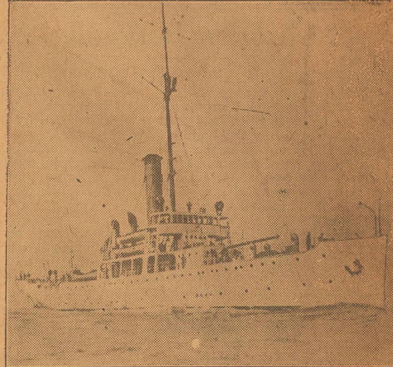
WORLD'S FIRST ELECTRIC COAST GUARD CUTTER —The Tampa, the world's first electric Coast Guard cutter, has been given her official sea trials off the Pacific coast. She exceeded her speed requirements, making 16.26 knots per hour. She has a 2,600 horse power motor.
