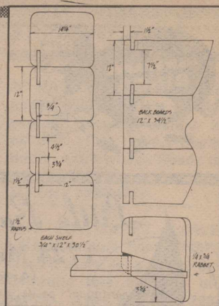
This diagram shows you how to fit pieces of the project together to form a sturdy bookcase that can be dismantled and moved whenever and wherever you will.
