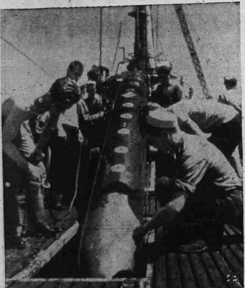
ELECTRIC 'TIN FISH' IS STOWED AWAY —Members of a U.S. Navy submarine crew stow an electric torpedo below decks. Just released by the navy, the "tin fish" is one of a type which accounted for 1,000,000 tons of enemy shipping in the war. Over 20 feet long, its gyroscopically-controlled progress through the water leaves no tell-tale wake. (AP Wirephoto from U.S. Navy).
