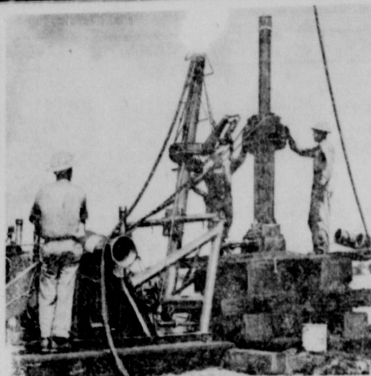
PULLING UP STAKES—Old pipe is being used to drill new oil wells nowadays. Oil companies, unable to obtain sufficient new pipe for full-time drilling operations, are going deep into the earth to recover from producing wells pipe that has been in service for as many as 30 years. Above, workmen pull out the pipe to put in a new well.
