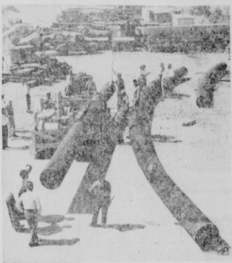
BIG BENDER —This powerful, portable machine bends cold oil and gas pipe with the greatest ease. The invention of John Coody of Houston, Tex., is able to bend perfect curves in pipe lines as big as 31 inches in diameter. S. M. Butler, who will manufacture the machine with Ole and Weed Peterson, said the bender will also fit pipe lines to any terrain without leaving wrinkles on the inside of the pipe. (AP Photo)
