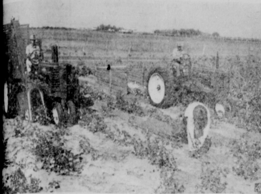
OLD AND THE NEW IN COTTON PICKING —Contrasting methods of harvesting cotton in the Pecos Valley are shown above at the National Cotton Council's second annual Beltwide Cotton Conference at Lubbock, Tex., Oct. 14. The modern, tractor-powered, two-row cotton picker shown at the left can harvest a bale of cotton in 30 minutes; the handpicker gathers a bale in about 20 hours when drawn by a tractor.
