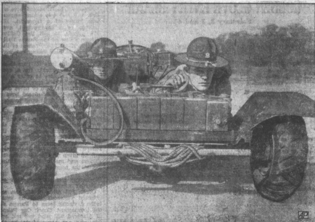
GETTING DOWN TO EARTH , Corp. Berry W. Russell (right) and Machine Gunner Tom M. Newberry manned the U. S. army's new low-slung Howie machine gun carrier during a demonstration at Fort Benning in Georgia. Steered by a handle, the iron raft is accelerated by foot pedals. Its advantage rests in the prone position of the two men, offering a poor target. The carrier, which easily worked its way over rough ground during the demonstration, weighs a little more than half a ton and can scoot along at better than 28 miles an hour. Its inventor is Capt. Robert G. Howie.
