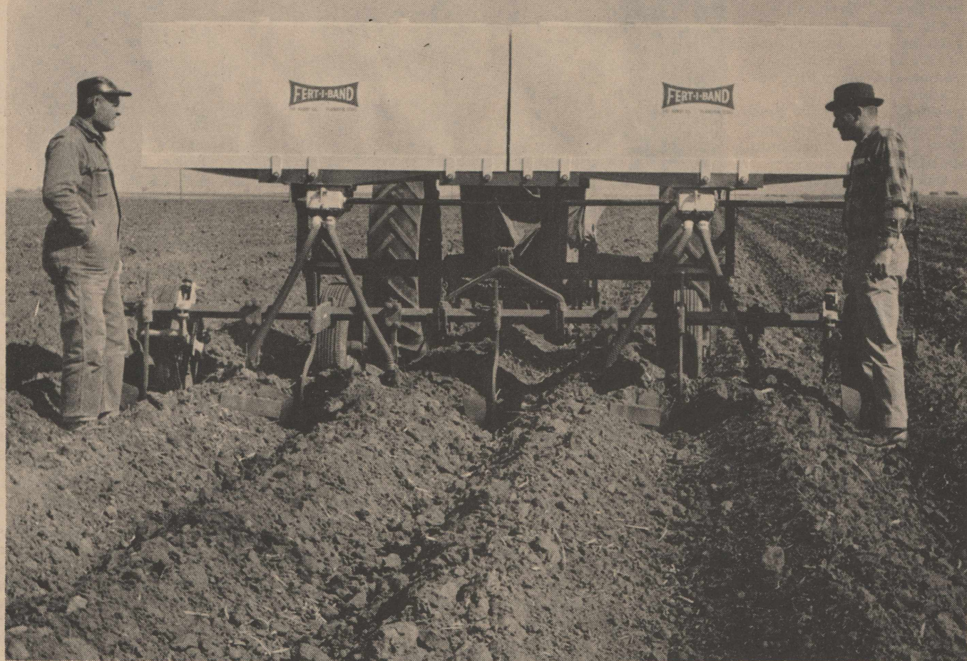
DON SPAIN AND DUDE HARMON INSPECT NEW BANDING MACHINE WHICH APPLIED AMMO-PHOS 11-48-0 AT FLOYD BANNISTER FARM THIS WEEK
