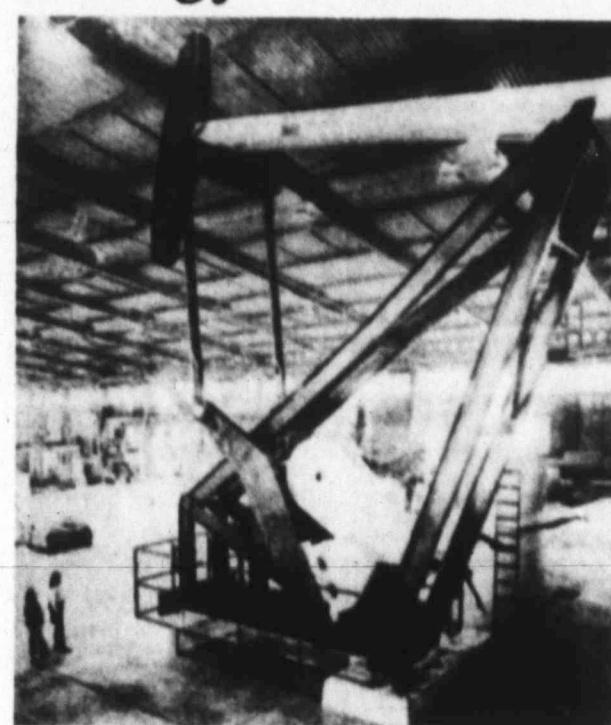
BIGGEST UNIT — The Lutkin Mark II pumping unit, the world's largest crank counterbalanced unit, is on display at the International Petroleum Exposition this week in Tulsa, Okla. It is capable of producing up to 9,000 barrels of fluid a day.
