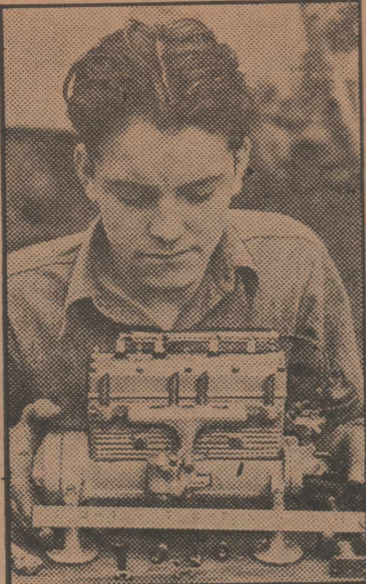
A "baby" motor ten inches long and seven inches high, is pictured above, displayed by its young builder, Lathiel Morris, Jr., of Venice, Calif. Product of a year's work, the tiny aluminum engine is a four-cylinder, four cycle, L-type, with one-sixteenth bore and one-sixteenth stroke. The lad plans to install it in his 39-inch, radio-controlled motorboat.
