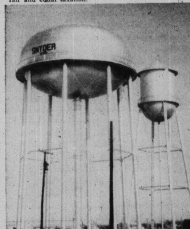
STORAGE DOUBLED LAST YEAR —With the installation of this 500,000 gallon elevated storage tank last August, the elevated water storage capacity of the city was doubled. While improving water service in the southwest part of the city, it also accounted for a two cent reduction in the fire insurance key rate for Snyder citizens.
