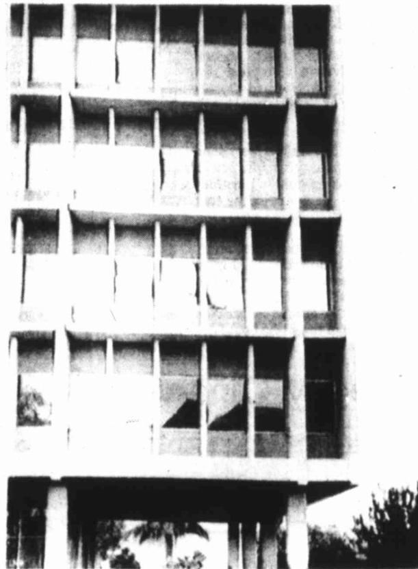
EXTENSIVE STRUCTURAL DAMAGE — The Imperial County General Services Building is tilting from the force of an earthquake that struck southern California at 4:18
