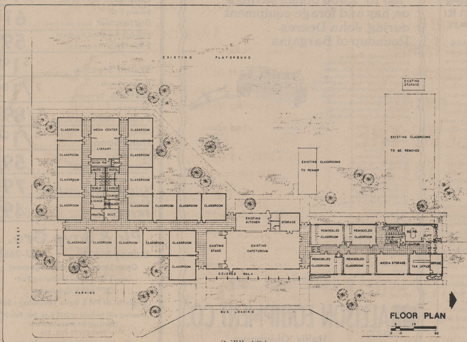
Floor plan of proposed Elementary School.
