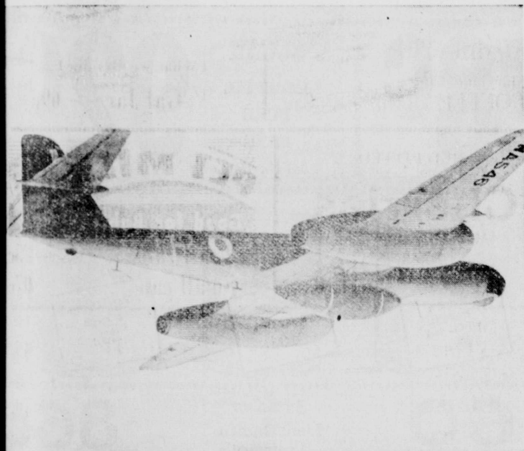
FLYING RADAR STATION —This is the first air-to-air photo of the new Armstrong Whitworth F-11, probably the world's fastest jet-propelled night fighter plane, unveiled in England. The plane was designed especially to prevent an atomic Pearl Harbor in Europe and its elongated nose contains the latest radar equipment. Note the ventral fuel tank under the fuselage.
