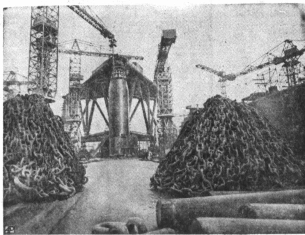
'SEA QUEST' LAUNCHED — "Mechanical birds" (cranes) and ships' chain frame scene at launching of drilling platform at Belfast, Northern Ireland. The 3-legged rig, built to stand above 60-foot waves, will search for oil and gas under North Sea.
