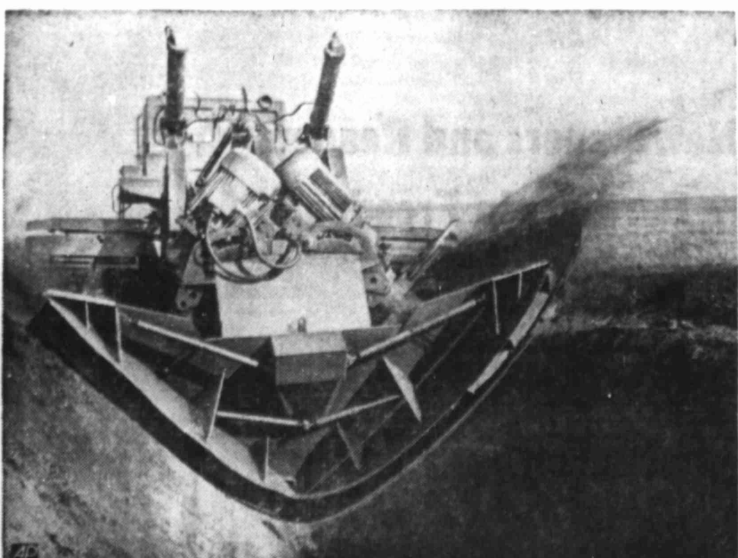
SOVIET CANAL CUTTER — A new canal and ditch digger, the KFN-1200 now in production in Byelorussia, is designed to dig irrigation canals. Depending on type of soil, the tractor-hauled machine can cut a 4-foot trench at 100 to 865 feet per hour.
