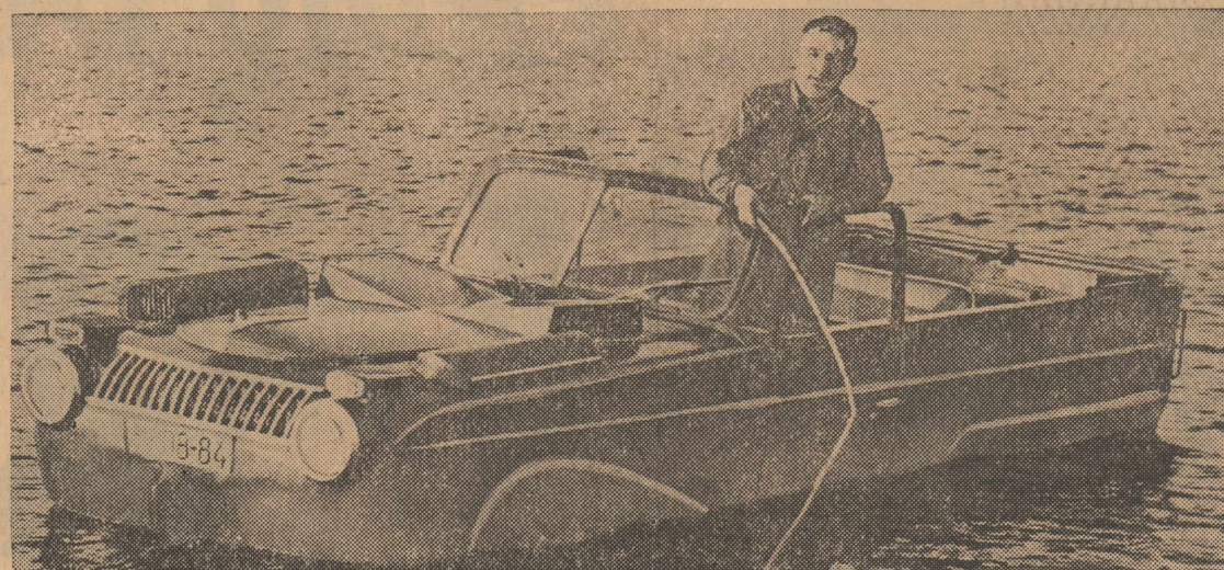
FISHY STORY—Grigori Khokhlov threw his line overboard from his car, which he designed himself. The amphibious car, which will travel over the rough roads in Novosibirsk, in Siberia, and which will also take to the water has a motor which runs the four-wheel drive and propeller. This photograph is from an official Soviet source.
