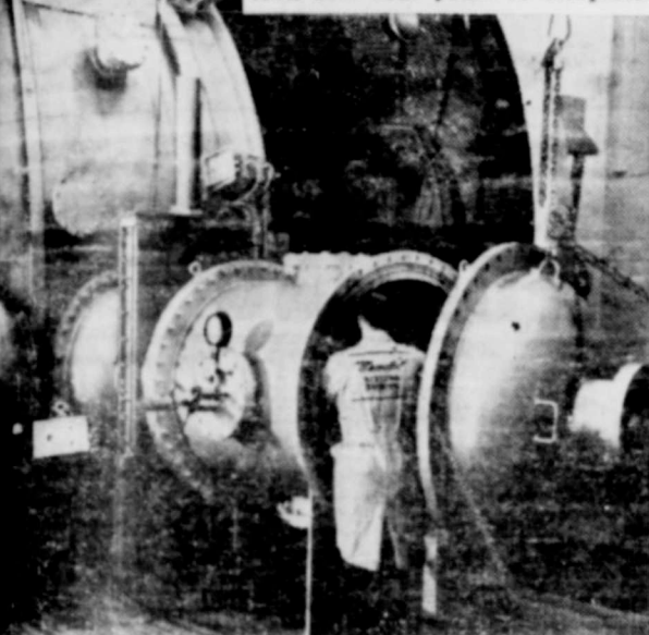
SPACE CHAMBER attached to "mother" is tended by ... in what is believed to be only facility of its kind in ... Designed by Bendix Systems division engineers, the ... chamber duplicates atmospheric pressure changes ... by a rocket-borne payload as it zooms into space.
