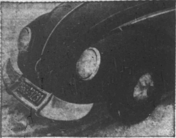
ROAD-HUGGING DEVICE —A former airplane maker in Munich, Germany, developed this "asloran," designed to keep the car glued to the road at high speeds. Using aerodynamic principles, the asloran, mounted where the front bumper used to be, causes air flowing over it at high speeds to add to front-end "weight" of the auto, keeping it stable at high speeds. Device sells for about $25.
