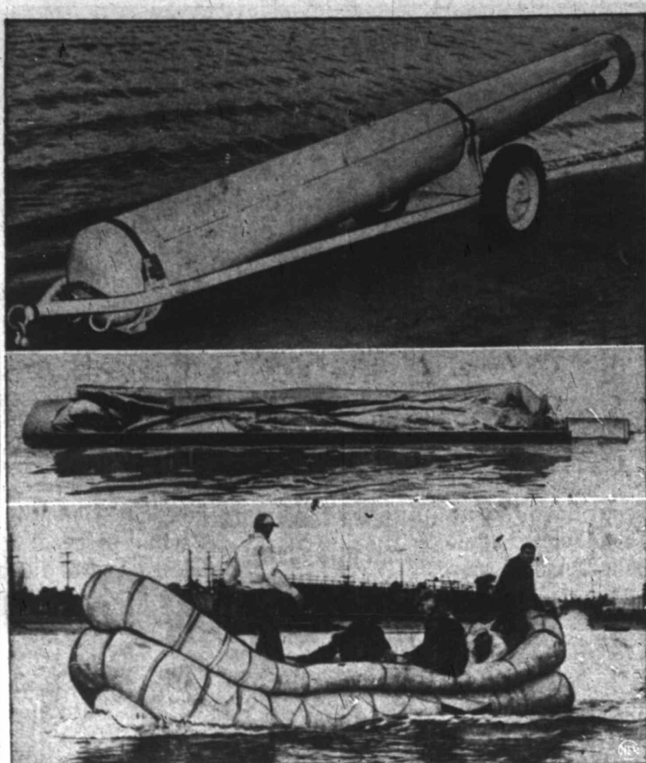
NEW "TORPEDO BOAT" IS AIR-SEA RESCUE CRAFT —Torpedo-like in appearance, the new air-sea rescue device unveiled by Douglas Aircraft at Long Beach, Calif., is a highly versatile rescue raft. Top view shows the aluminum alloy cylinder, 20 feet long and 21 inches in diameter, that contains self-inflating raft, four-cylinder engine with radio controls and food and survival equipment for eight occupants for five days. Middle view shows raft beginning to inflate automatically within two minutes after launching. Bottom view shows fully-inflated raft being propelled by its engine. The craft, developed by Douglas and the Air Force's Air Materiel Command, can be launched and steered by remote radio control from a plane or any ocean craft that is equipped with torpedos tubes.
