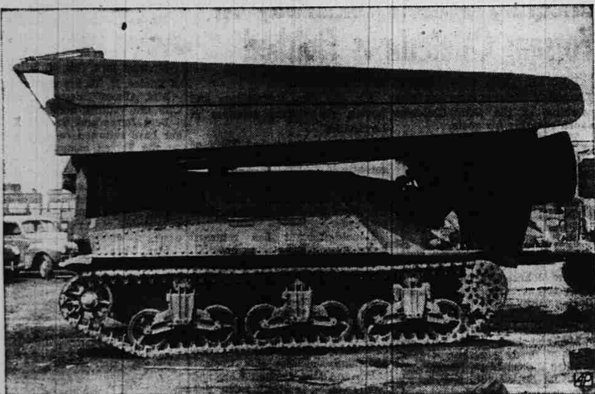
TANK CARRIES BRIDGE —This tank-carried bridge, developed by Gar Wood Industries and the Army, opens like a scissors on a heavy hinge to span distances up to 37 feet.
