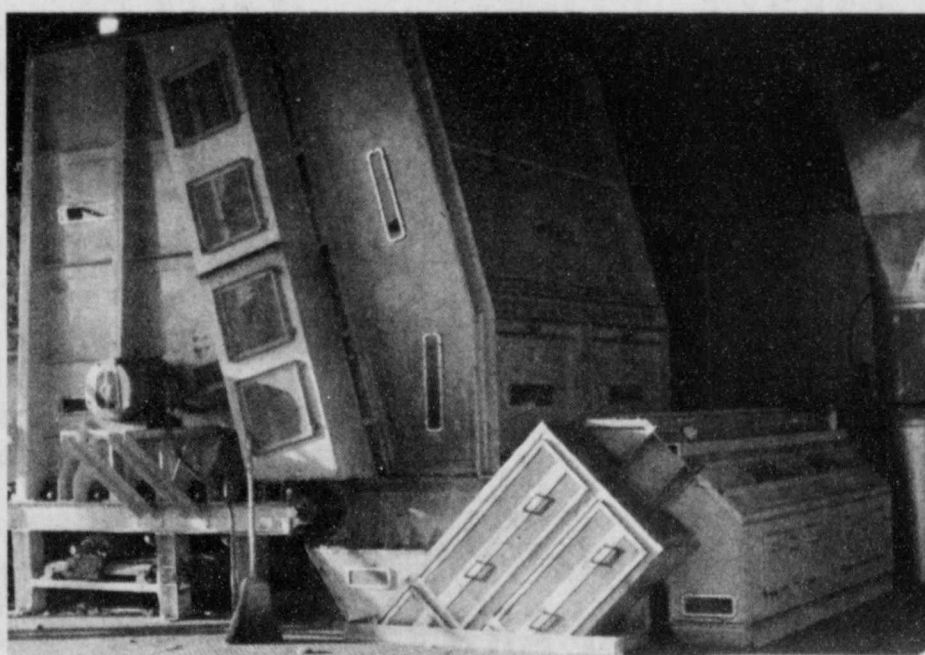
THE FEEDER HEAD THEN SEPARATES THE TRASH FROM THE COTTON
