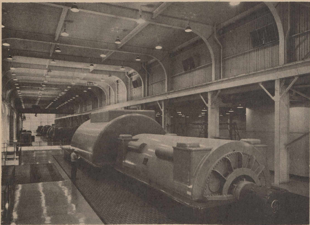
THE TURBINE ROOM--at Southwestern Public Service Company's Plant X, in Lamb County near Earth, now houses four giant electric generators, with a capability of 487,500 kilowatts. The turbo-generator in the foreground, with a capability of 210,000 kilowatts, is the largest single generating unit now in service on the electric company's system. The length of the turbine room floor is 522 feet, nearly the length of two football fields.
