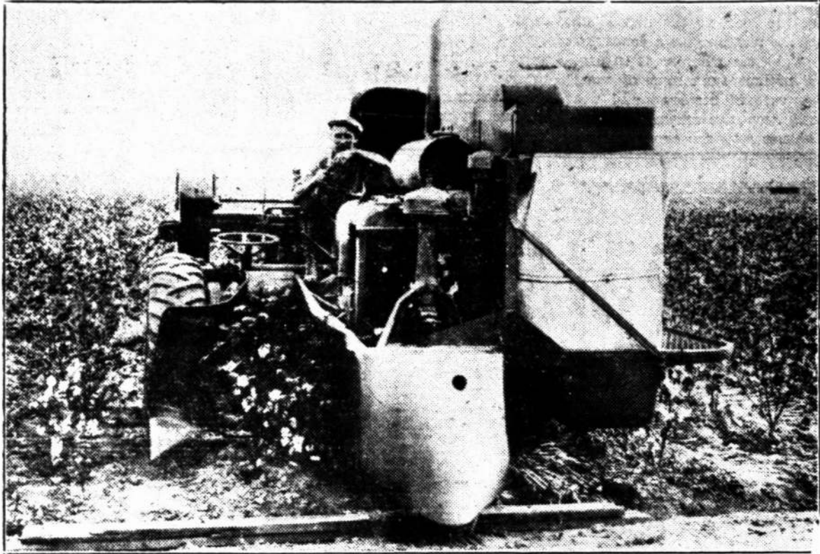
Front view of a 1936 model McCormick-Deering Farmall cotton picker with cleaner, on Hopson Plantation, Clarksdale, Mississippi. The machine is of the spindle type.
